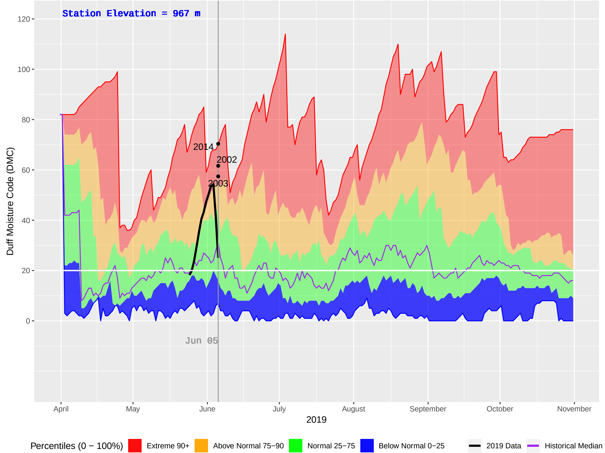
WONOWON (136) : Historical (1990–2018), Current (2019) Daily Duff Moisture Code (DMC)
