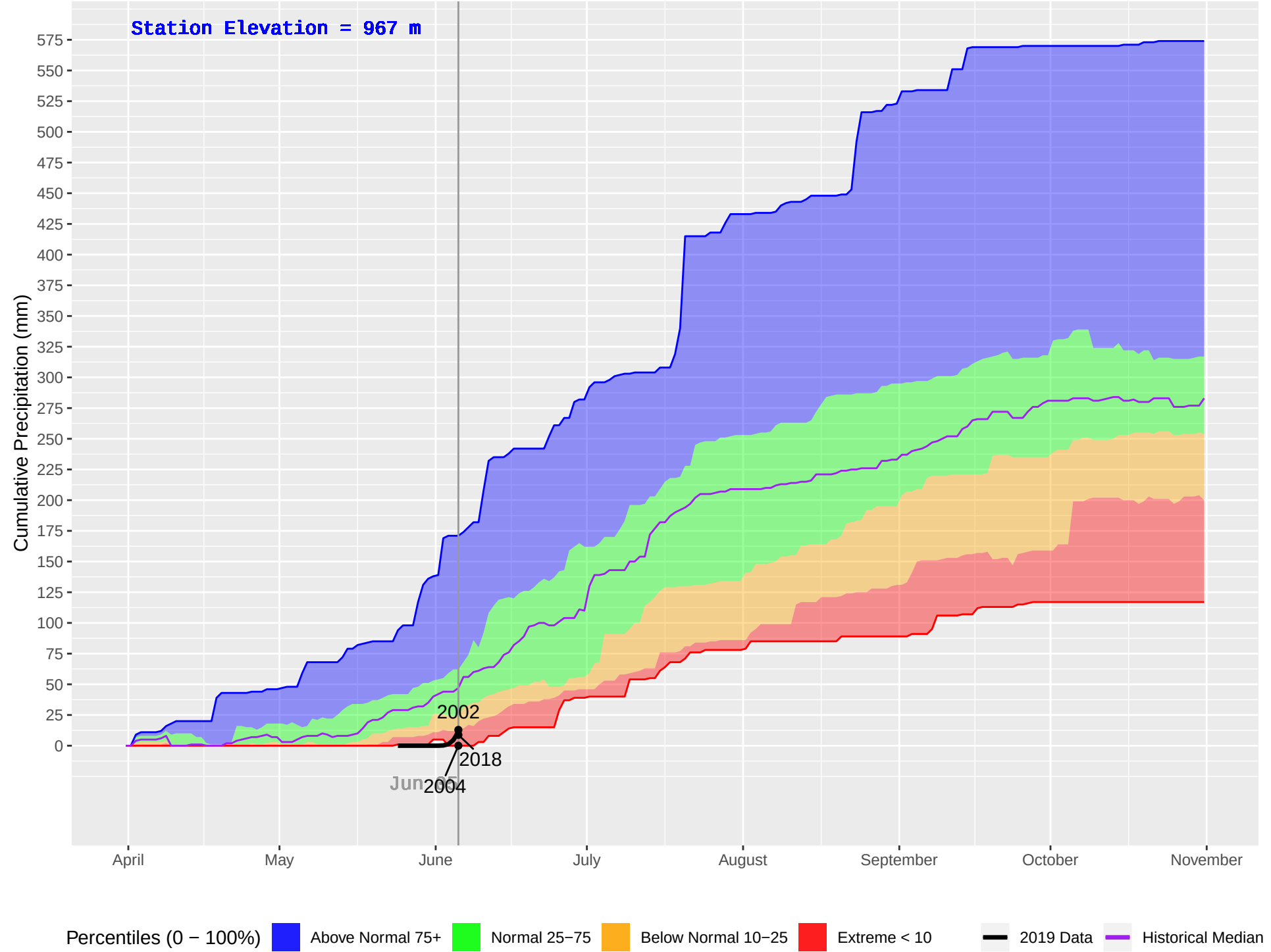
WONOWON (136) : Historical (1990–2018), Current (2019) Daily Cumulative Precipitation
