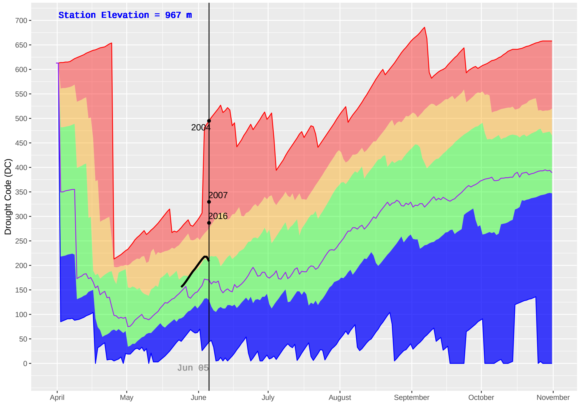
WONOWON (136) : Historical (1990–2018) and Current (2019) Daily Drought Code (DC)
