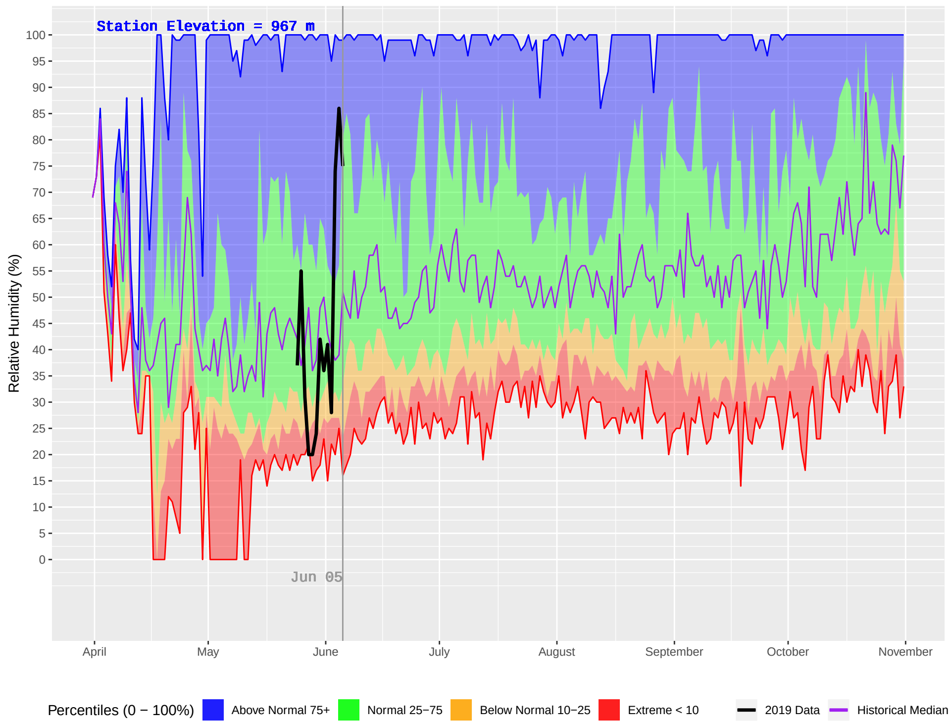
WONOWON (136) : Historical (1990–2018) and Current (2019) Daily Relative Humidity
