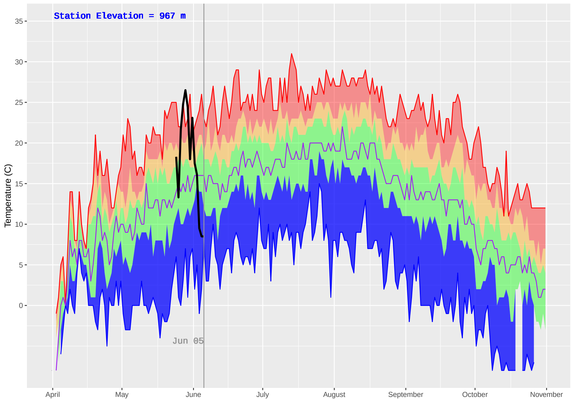
WONOWON (136) : Historical (1990–2018) and Current (2019) Daily Temperature
