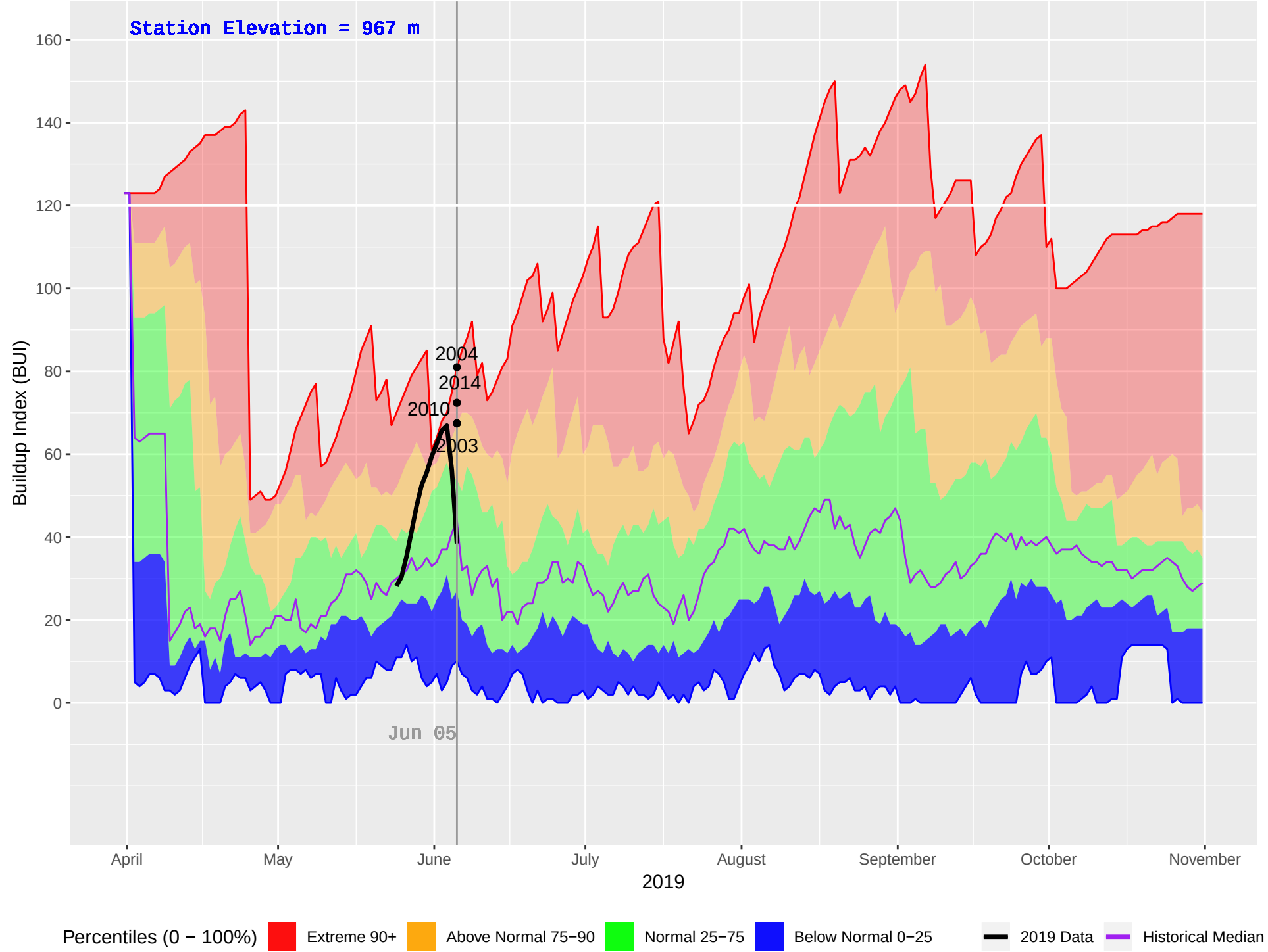
WONOWON (136) : Historical (1990–2018), Current (2019) Daily Buildup Index (BUI)
